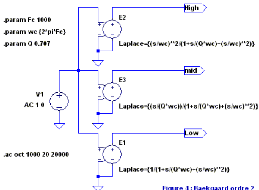
Figure 4: Baekgaard ordre 2
