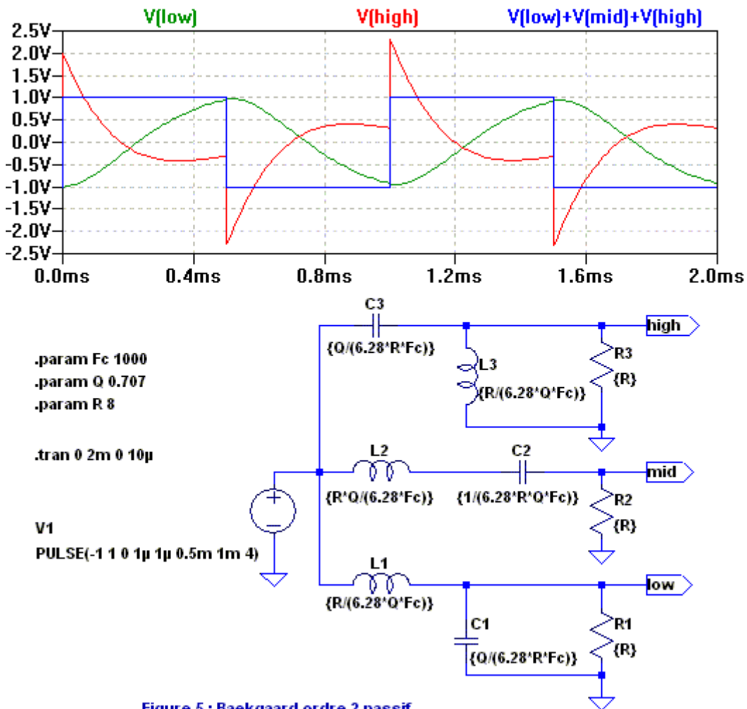
Figure 5 : Baekgaard ordre 2 passif
